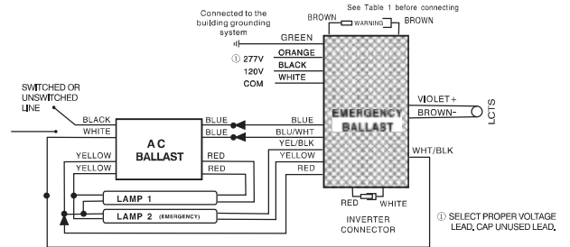
B. TWO (2) LAMP RAPID START BALLAST
