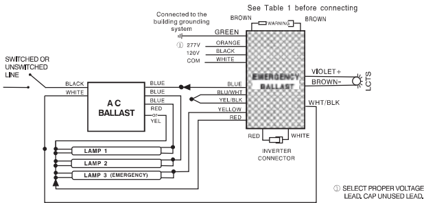
G. THREE (3) LAMP INSTANT START BALLAST
