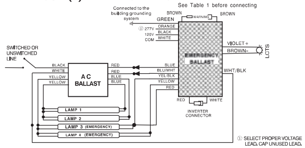
R. FOUR (4) LAMP INSTANT START BALLAST
