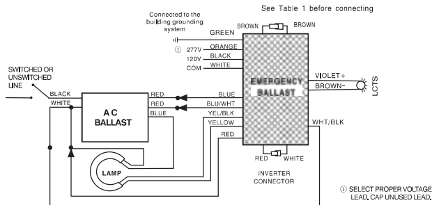
K. ONE (1) LAMP CIRCLINE RAPID START BALLAST
