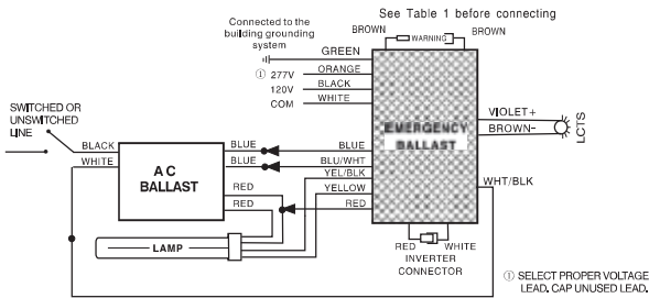
I. ONE (1) 4-PIN COMPACT LAMP RAPID START BALLAST
