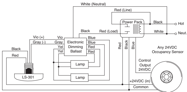
Wiring with Occupancy Sensor
