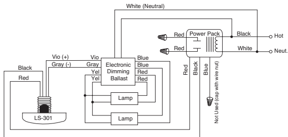
Typical Wiring
