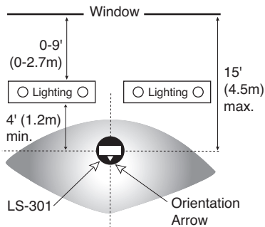
Fig.2: Placement in applications where lighting fixtures are within 10 feet (3m) of daylight source
