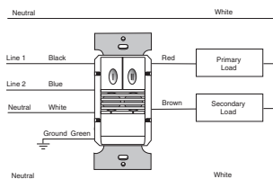
DSW-200 Dual Circuit Wiring
